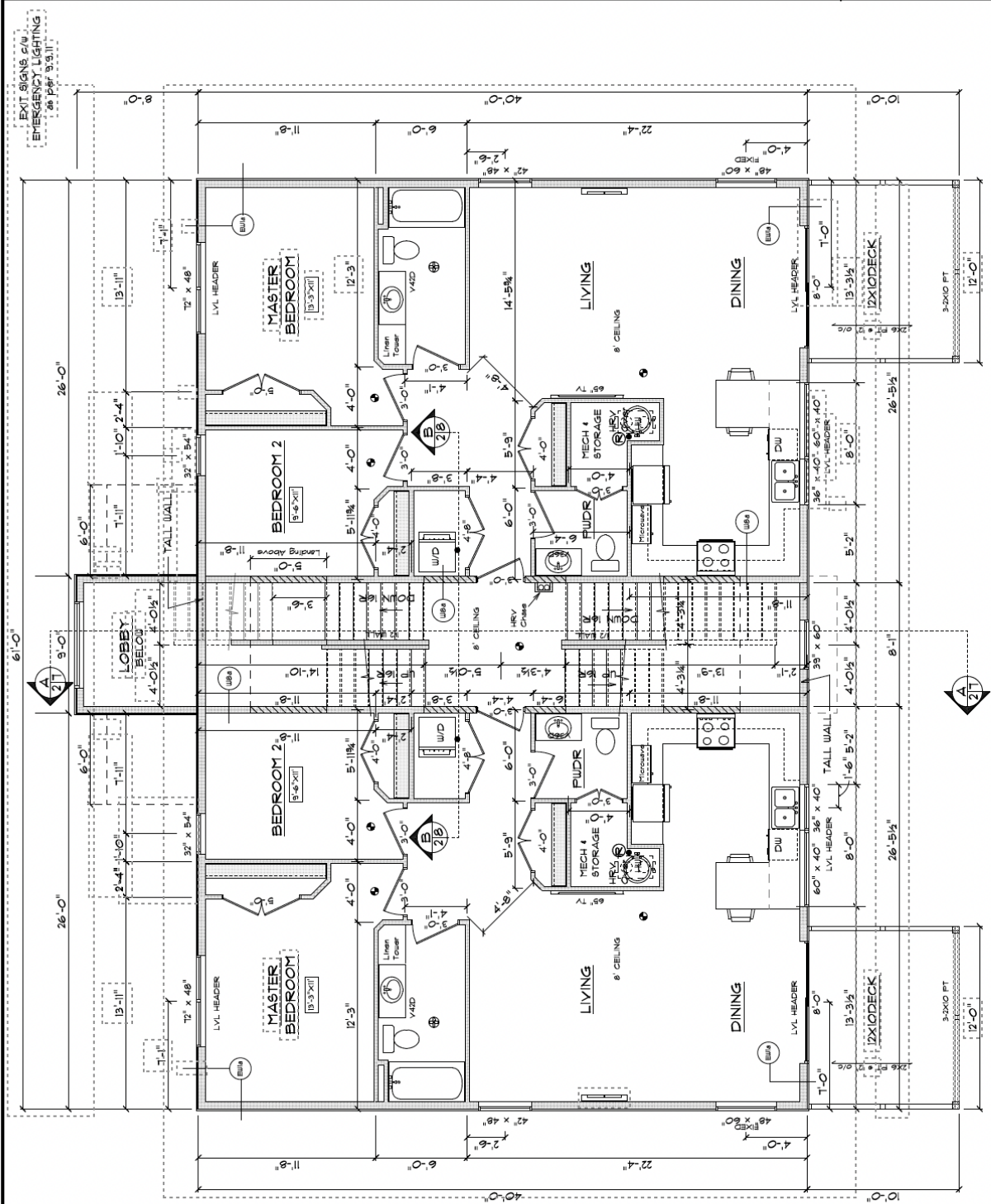
MEET ALL ADAPTABLE HOUSING REQUIREMENTS. 46 PER NBOR 3.8'4" INCLUDING BLOCKING FOR FUTURE BATHROOM GRAB BARS
